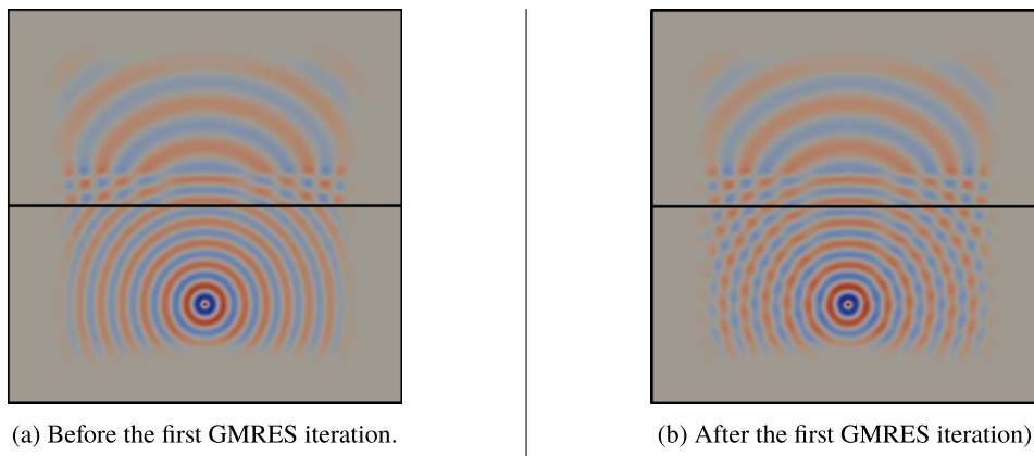
Fig. 20. Illustration of the computed wavefields.
