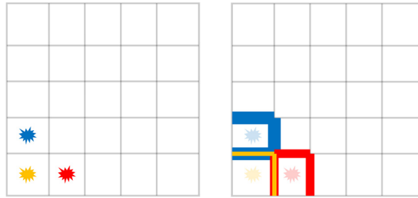
Fig. 11. Left: The setup of the problem in scenario 3, with multiple point sources shown in red, yellow and blue. Right: The extracted trace information is shown using the same colors as their corresponding point sources.
