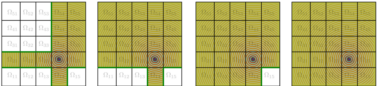
Fig. 10. The computed wavefield and traces (green) after each sweep in stage 3 of scenario 2.
