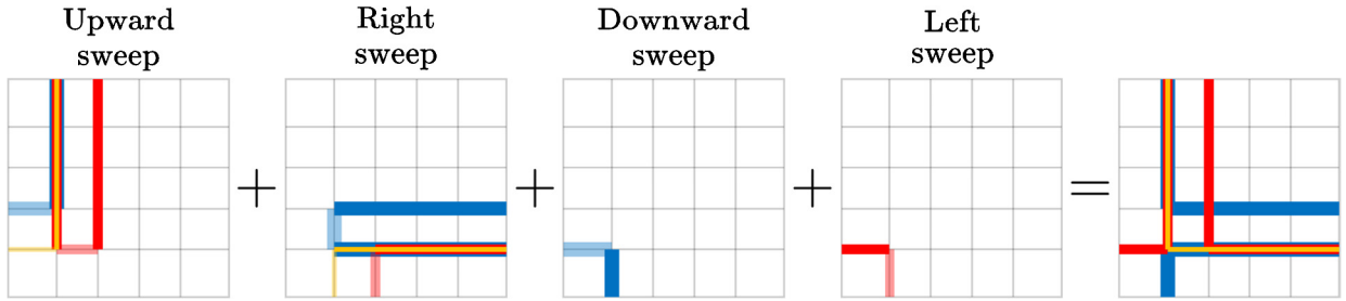
Fig. 13. The propagation of the trace information in each sweep of stage 2 of scenario 3. The stage 1 traces used in each sweep are shown in the light colors. The traces generated by stage 2 and used in stage 3 are shown in bold colors. The traces are color-coded with respect to the sources they originated from in Fig. 11.
