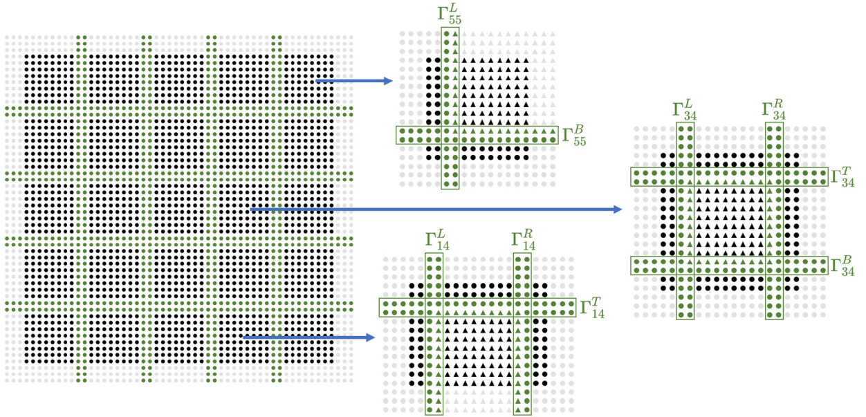
Fig. 16. Illustration of the discrete local problems and the discrete interfaces. Discrete interfaces are colored in green and degrees of freedom corresponding to the sets \Omega_{ij} are denoted by triangles.
