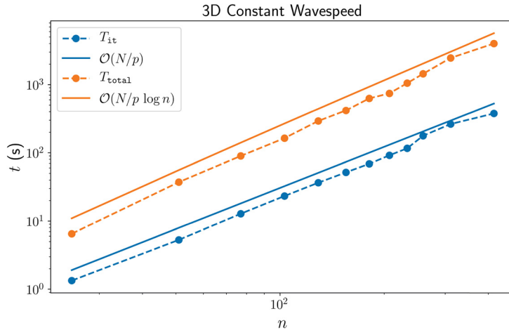
Fig. 27. Timings for the 3D experiment with constant wave speed. Solid lines are empirical complexities for one application of the preconditioner (blue) and for the over-all solve (orange). Dashed lines are with measured results for one application of the preconditioner (blue) and for the over-all solve (orange).
