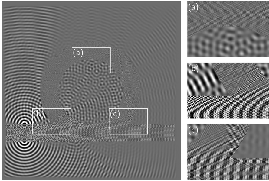
Fig. 26. The computed wavefield for a contrast ratio of 6 and \omega/2\pi = 323.1 . Zoom regions (a), (b), and (c) highlight solution quality in areas of high-contrast in the wave speed.
