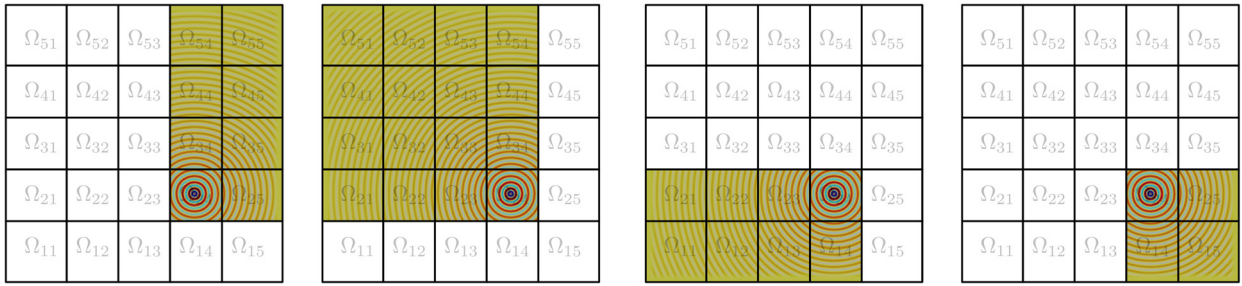
Fig. 8. The solutions in each quadrant in scenario 2.
