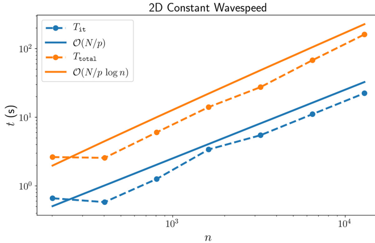
Fig. 21. Timings for 2D experiment with constant wave speed. Solid lines are empirical complexities for one application of the preconditioner (blue) and for the over-all solve (orange). Dashed lines are with measured results for one application of the preconditioner (blue) and for the over-all solve (orange).
