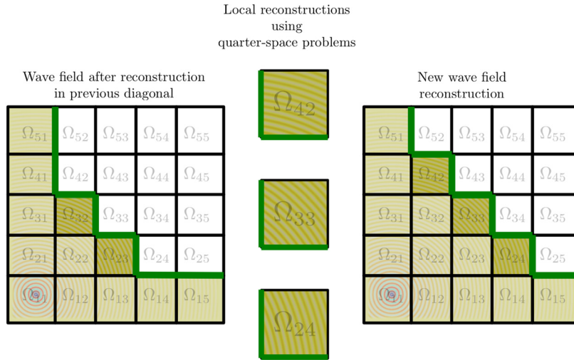
Fig. 6. Summary of the computed solution in one diagonal sweeping step. Updated subdomains are diagonally adjacent in a direction perpendicular to the bottom-left to top-right sweep direction.
