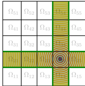
Fig. 9. The computed wavefield and traces (green) after stage 2 of scenario 2.
