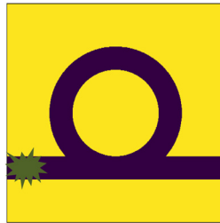
Fig. 25. The wave speed distribution of the wave-guide. The point source at the entrance is shown by the green star.
