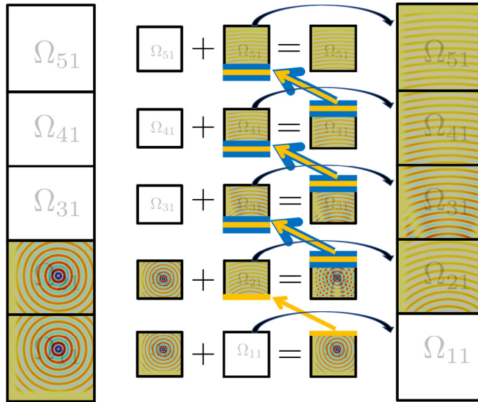
Fig. 12. Summary of the upwards sweep, for scenario 3, in one column in the presence of several point sources.
