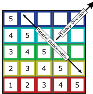
Fig. 18. Illustration of parallelism in diagonal sweeps. Subdomains processed in parallel have same label. Subdomains with like color are assigned to same processor.
