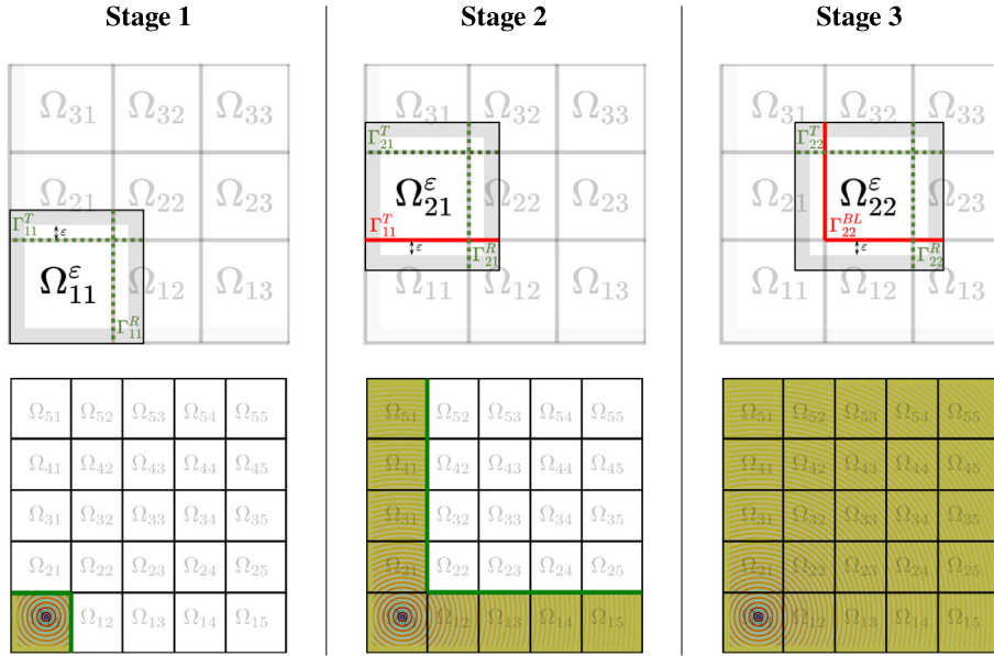
Fig. 5. Illustration of local problems (top row) and the computed solution after each stage of a sweep (bottom row). The green lines in the wavefields depict extracted trace information used in the next stage.
