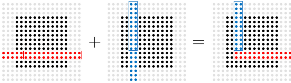
Fig. 17. Illustration of the construction of the discrete L-shaped trace.
