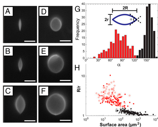
Fig. 2. Characterization of the two populations of GUVs that formed in nematic DSCG. Fluorescence micrographs of (A–C) highly elongated, cusped GUVs and (D–F) weakly strained GUVs with approximately rounded poles. (G) Histogram depicting the distribution of cusp angles ( \alpha ). (H) GUV aspect ratio ( R/r ) as a function of GUV surface area. In G and H, data in red and black denote GUVs with \alpha < 130^\circ and \alpha > 130^\circ , respectively. In H, filled and open points denote GUVs containing 2 mol % PEG lipid and 0.2 mol % PEG lipid, respectively. (Scale bars: 5 \mu\text{m} .)
