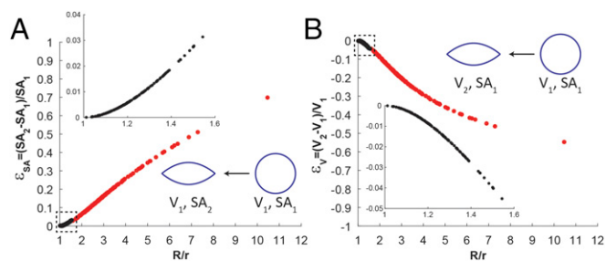
Fig. 3. Fractional changes in surface area and volume calculated to accompany LC-induced GUV shape transformations. (A) Fractional GUV surface area expansion ( \varepsilon_{SA} ) calculated for an LC-induced GUV shape transformation at constant internal GUV volume. (B) Fractional change in GUV internal volume ( \varepsilon_V ) calculated for an LC-induced GUV shape transformation at constant GUV membrane surface area. Data in red denote GUVs with cusp angles \alpha < 130^\circ , and data in black denote GUVs with cusp angles \alpha > 130^\circ .
