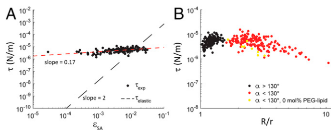
Fig. 4. Plots of \tau as a function of fractional GUV surface area expansion ( \epsilon_{SA} ) and GUV aspect ratio ( R/r ). (A) Log-log plot of \tau_{exp} as a function of \epsilon_{SA} for the population of GUVs with \alpha > 130^\circ . The slope of a power law fit to the data is indicated. The relationship between \tau_{elastic} and \epsilon_{SA} is also shown. (B) Log-log plot of \tau_{exp} as a function of R/r . Data in red and black denote GUVs with cusp angles \alpha < 130^\circ and \alpha > 130^\circ , respectively, prepared with 0.2–2 mol % PEG lipid. Data in yellow denote GUVs prepared with 0 mol % PEG lipid, all of which had \alpha < 130^\circ .
