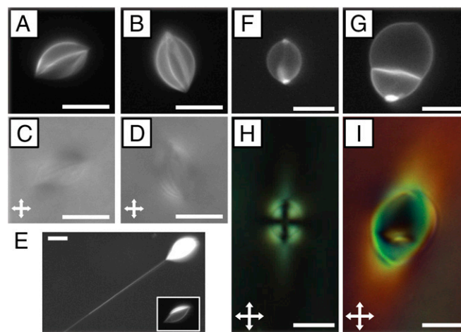
Fig. 5. Examples of complex GUV shapes and behaviors observed in nematic phases of DSCG. (A and B) Fluorescence micrographs and (C and D) corresponding optical micrographs (crossed polarizers) of wrinkled GUVs containing 2 mol % PEG lipid GUVs [15% (wt/wt) DSCG at 25 °C]. (E) Fluorescence micrograph of a GUV with a lipid tube extending from its pole. E, Inset is a micrograph collected using a shorter exposure time. (F and H) Fluorescence and crossed polar micrographs, respectively, of a GUV with polar regions exhibiting enhanced fluorescence signals. (G and I) Fluorescence and crossed polar micrographs, respectively, of two GUVs that are either fusing or budding. Details are in the text. (Scale bars: 10 \mu\text{m} .)
