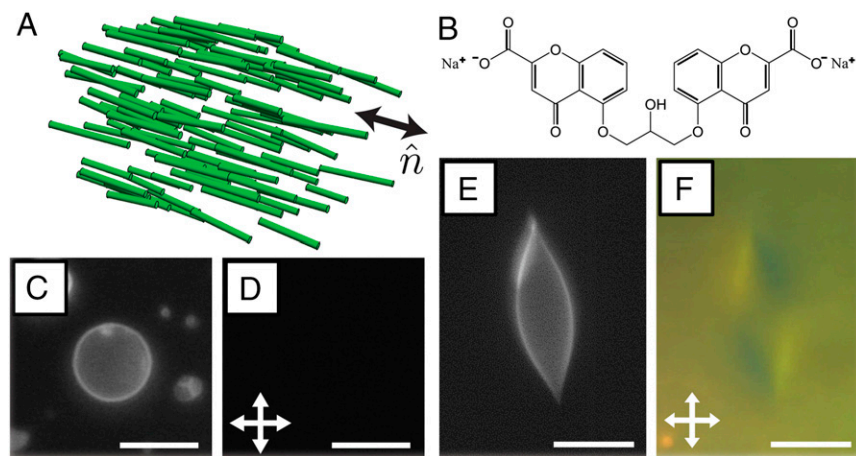
Fig. 1. (A) Schematic illustration of the long-range orientational order of a nematic LC, which can be characterized by a local director \hat{n} . (B) The chemical structure of a DSCG molecule. (C and E) Fluorescence and (D and F) crossed polar micrographs of GUVs in 15% (wt/wt) DSCG at (C and D) 48 °C (isotropic phase) and (E and F) at 25 °C (nematic phase). (Scale bars: 10 \mu\text{m} .)
