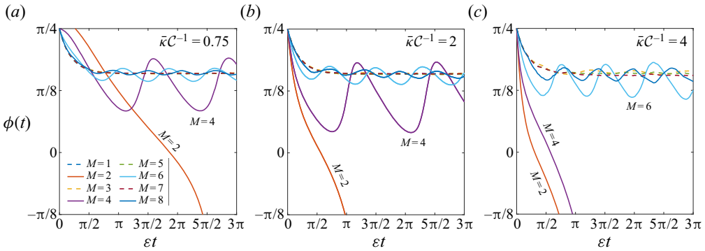
Figure 6. Inclination angle dynamics with bending stiffness variations in the M th spatial mode for M \in \{1, 2, \dots, 8\} with \epsilon = 0.1 or R_A = 0.865 and \lambda = 1 for three variation amplitudes, from the full numerical simulations. (a) \bar{\kappa}C^{-1} = 0.75 , (b) \bar{\kappa}C^{-1} = 2 and (c) \bar{\kappa}C^{-1} = 4 . Tumbling is observed in small, even modes. (See also supplementary movies M4–M6.)
