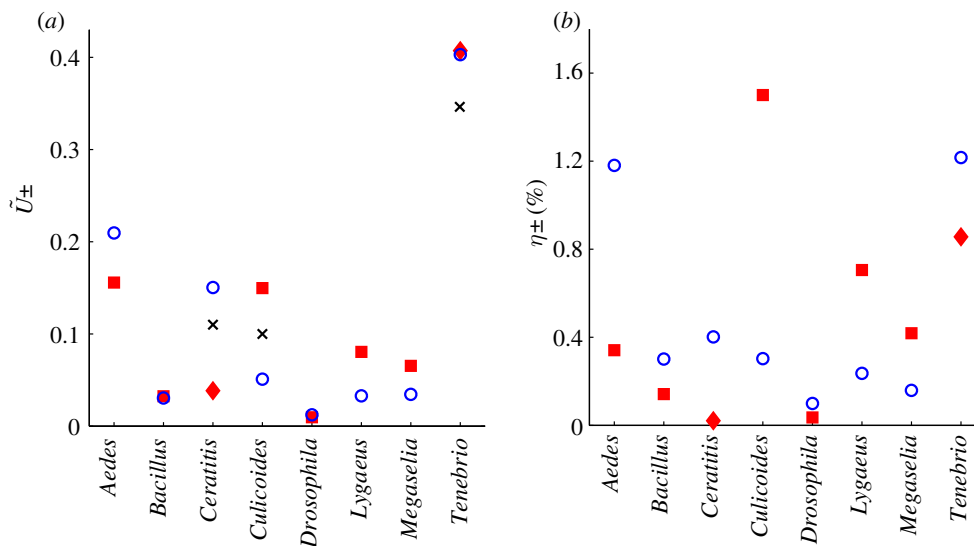
Figure 5. Predicted swimming performance: (a) average swimming speed, \tilde{U}_{\pm} , of different species; (b) hydrodynamic efficiency, \eta_{\pm} , of different species. Open symbols (blue circles) represent the same-chirality configuration (+); filled symbols (red squares and diamonds) represent the opposite-chirality configuration (-); for blue open circles and red squares, swimming occurs in the opposite direction as the wave propagation; on the contrary, red diamonds represent the cases of opposite-chirality configuration where the velocity in the z -direction occurs in the same direction as the wave propagation; black crosses represent experimental measurements of V = V_{\text{sperm}}/c_m (see tables 1 and 2). (Online version in colour.)
