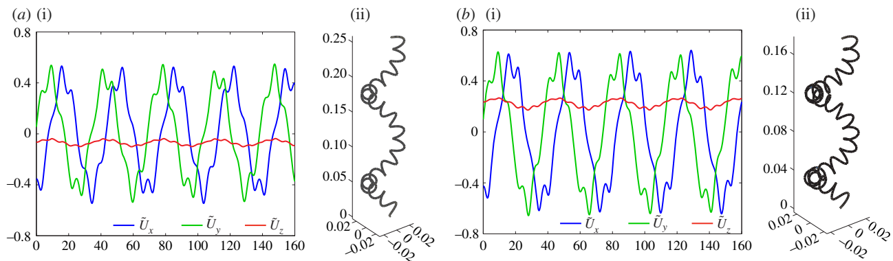
Figure 8. Three-dimensional swimming velocities in the laboratory frame (a(i), b(i)) of two opposite-chirality superhelical swimmers, and their corresponding geometries (a(ii), b(ii)). (a) R = 7 , r = 0.4 and U_z is negative, while the wave propagation is towards the positive z -direction; (b) R = 9 , r = 0.4 and U_z is positive, while the wave propagation is towards the positive z -direction. Geometric data of Cu. melleus spermatozoa are used for other parameters. (Online version in colour.)
