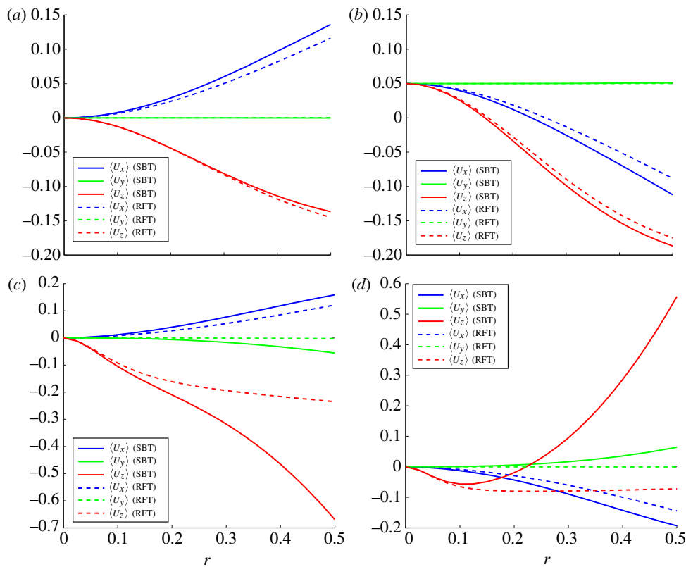
Figure 9. Comparison between the RFT (dashed lines) and the non-local SBT (solid lines) using geometric data of Cu. melleus spermatozoa ( a,b ), and T. molitor spermatozoa ( c,d ). The panels on the left (right) refer to the same- (opposite-) chirality configuration. (Online version in colour.)
