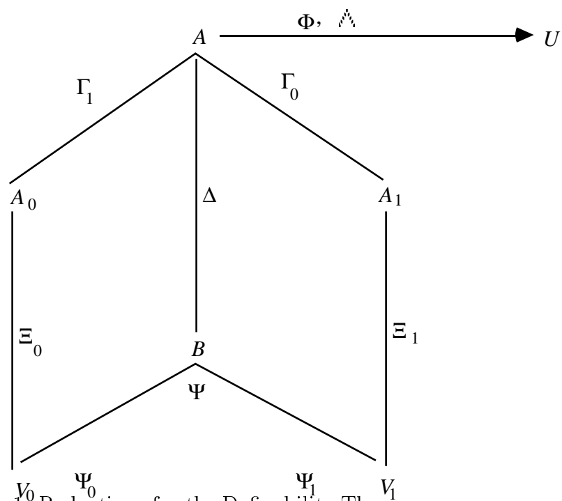
Figure 1: Reductions for the Definability Theorem
