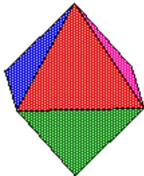
octahedron
