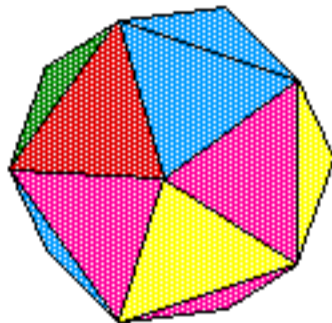
icosahedron
