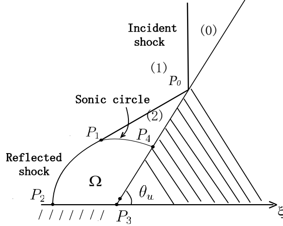
FIGURE 1. Regular Reflection Configuration
