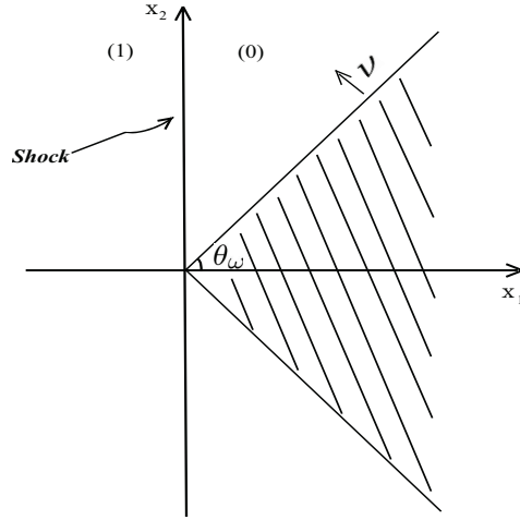
FIGURE 2. Initial-Boundary Value Problem
