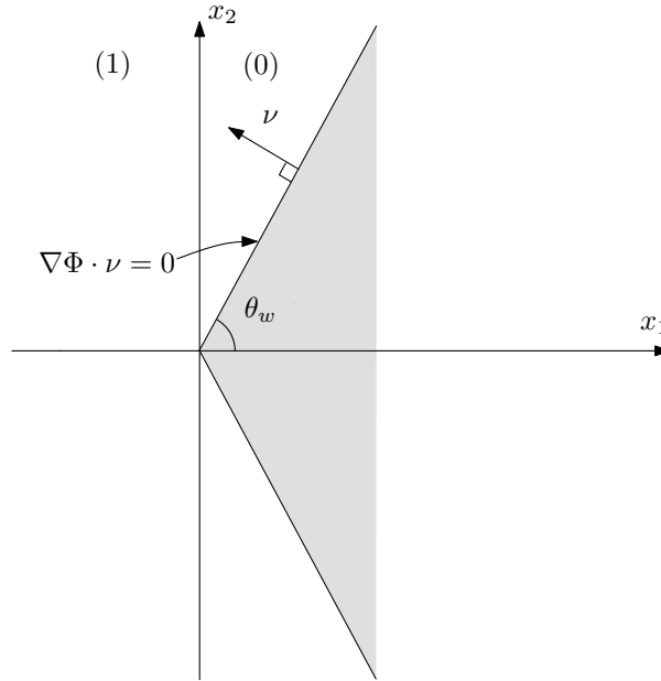
Figure 1.1: Initial-boundary value problem
