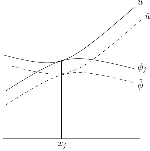
Figure 1: The subject of Jensen's Convolution.
