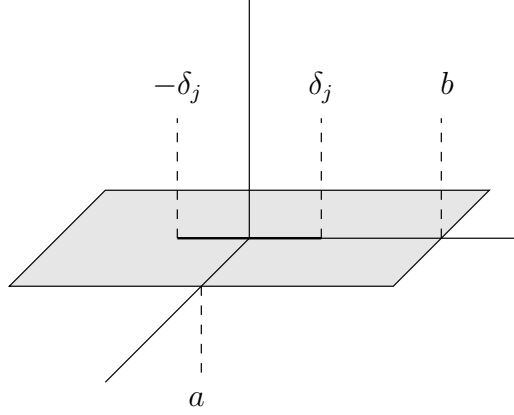
Figure 5: Rectangular domain for several of the latter cases.
