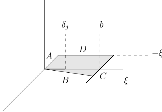
Figure 6: Modified domain for CASE 5.
