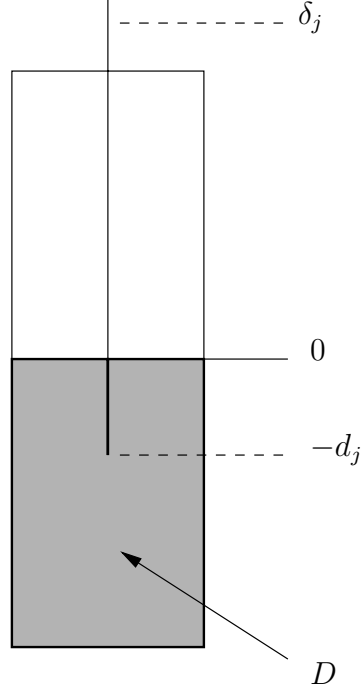
Figure 4: Rectangular domain along normalized sequence.
