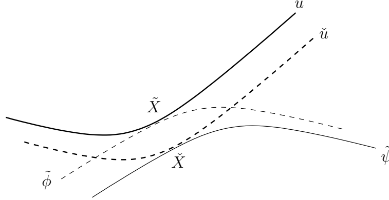
Figure 2: A twice differentiable point on Jensen's Convolution.
