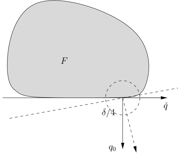
Figure 3: The neighborhood of an extreme point.
