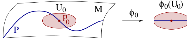
Figure 1.4: A coordinate chart adapted to a submanifold.
