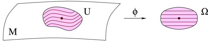
Figure 1.10: A foliation box.
