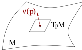
Figure 2.4: A unit normal vector field.
