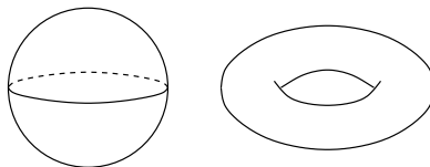
Figure 1.1: The 2-sphere and the 2-torus.
