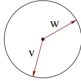
Figure 2.10: Two unit tangent vectors.
