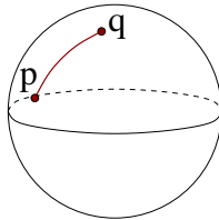
Figure 2.2: A geodesic on the 2-sphere.
