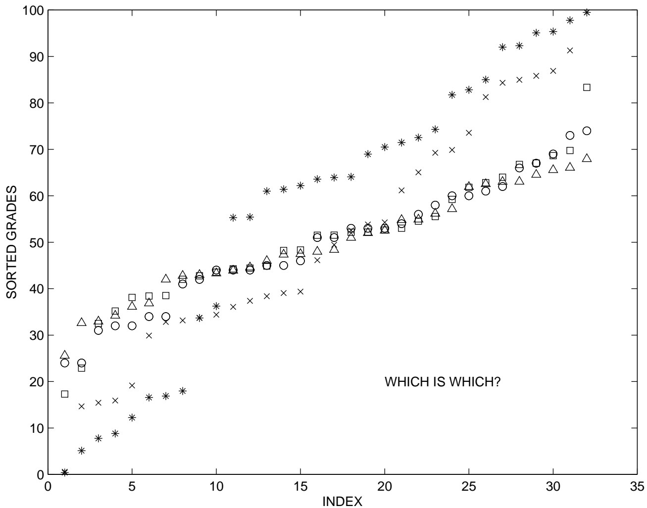
NEEP271 EXAM 1 GRADES vs. 2 random Gaussian and 2 uniform realizations
