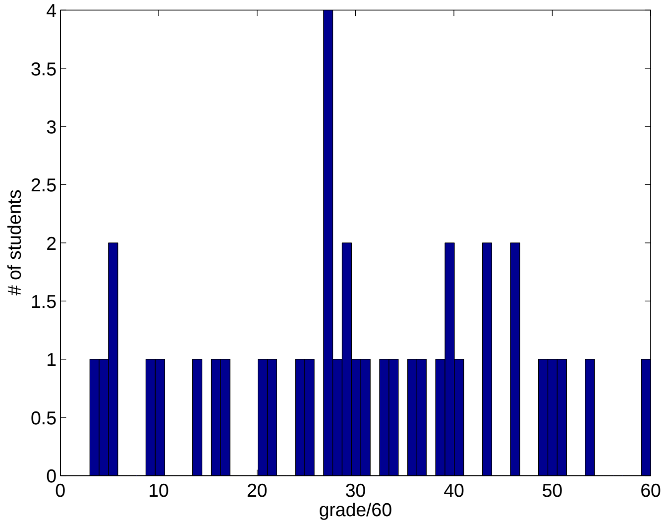
Math 321, Exam 2, Fall 2006
