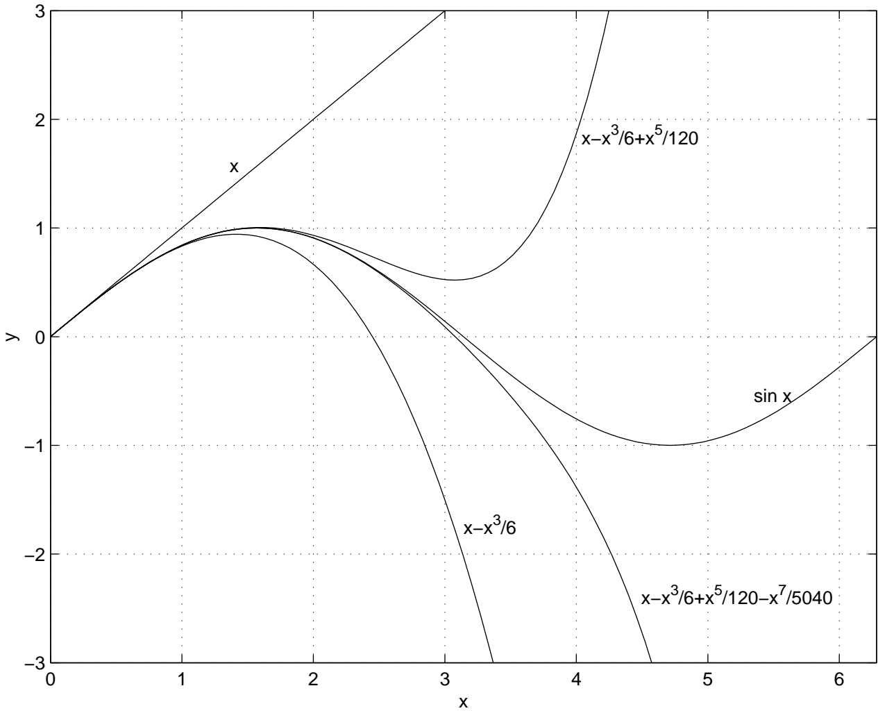
Polynomial approximations to sin(x) near x=0
