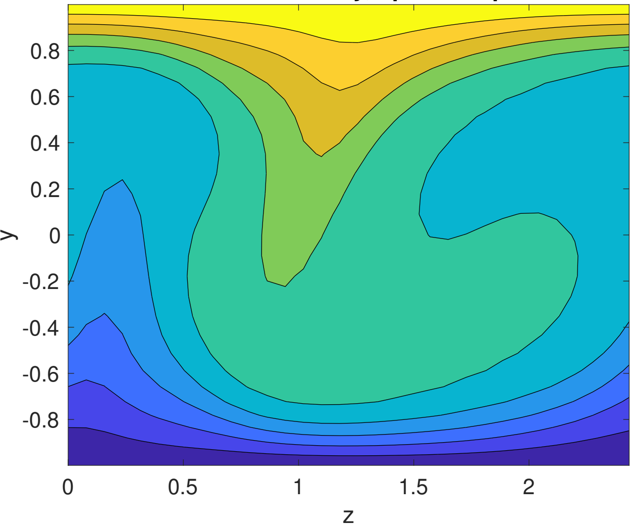
streamwise velocity, spanwise plane
