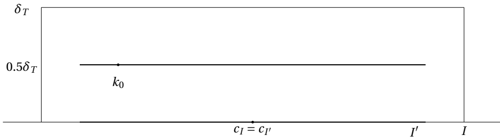
Figure 1: rectangle R_{I, \delta_T}
