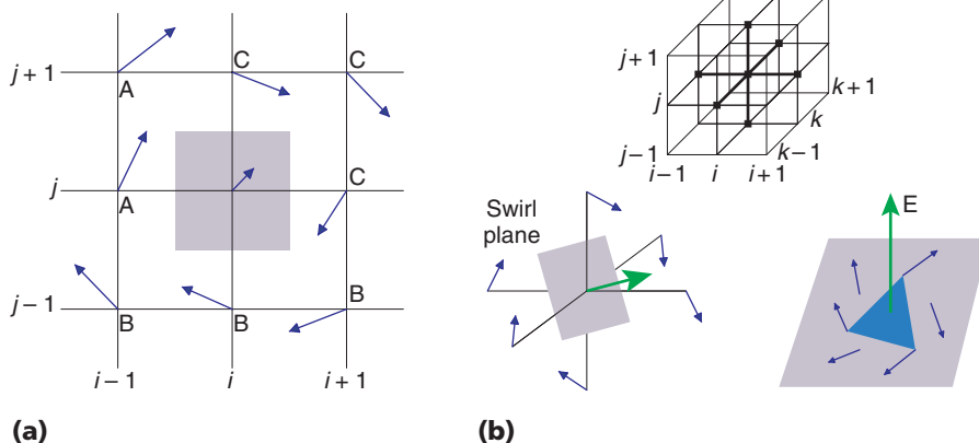
Figure 1. Topology-based vortex core region detection algorithm: (a) 2D algorithm and (b) 3D algorithm.
