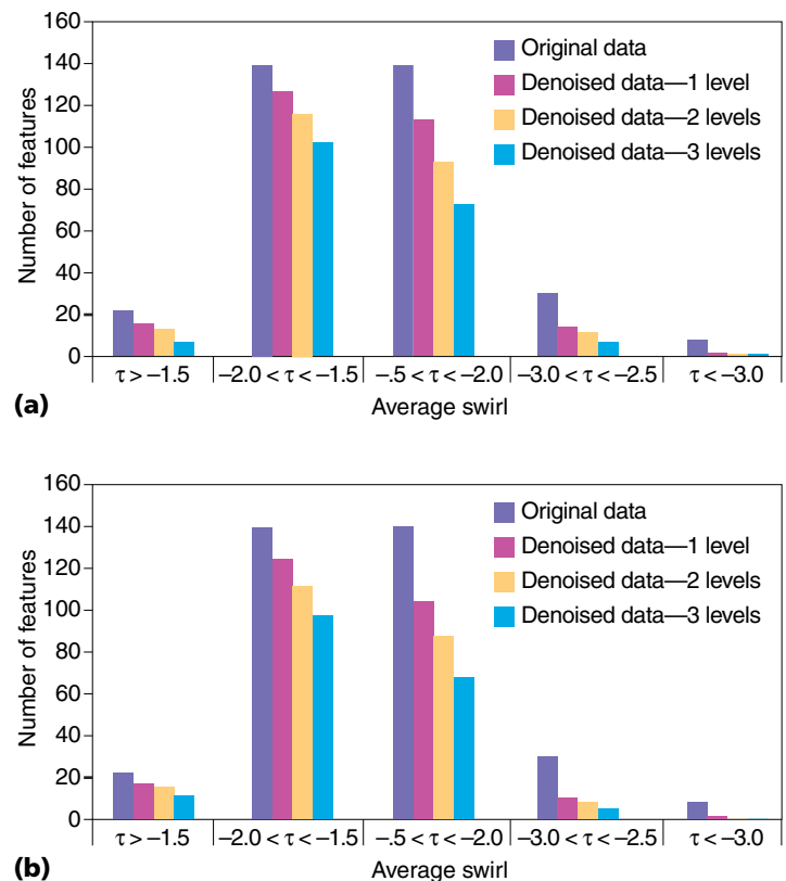
Figure 6. Denoising effectiveness based on average swirl: (a) linear lifting wavelet and (b) feature-preserving total variation diminishing wavelet.
