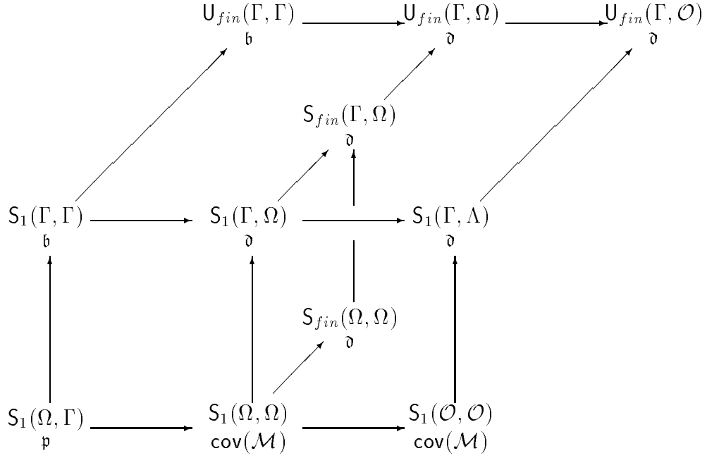
Figure 4: Cardinals \text{non}(P)
