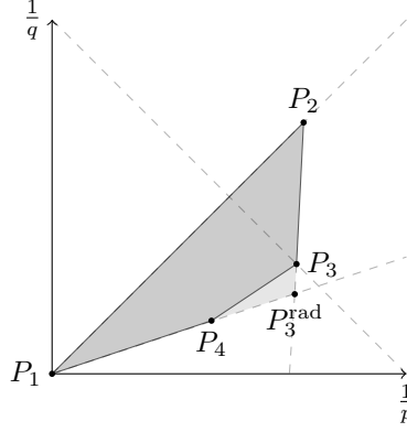
FIGURE 1. The triangle \Delta_\beta .
