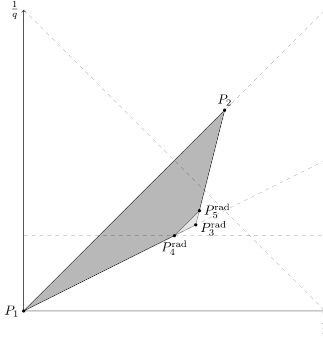
FIGURE 2. If d = 2, \beta = 0.5, \gamma = 1 , then \overline{\mathcal{T}_E^{\text{rad}}} is contained in \Delta_\beta and contains \mathcal{Q}_{\beta, \gamma}^{\text{rad}} . The condition 2\gamma - \beta > 1 says that the point P_3^{\text{rad}} = P_{3, \beta}^{\text{rad}} lies above the horizontal line q = 2(1 + \gamma) .
