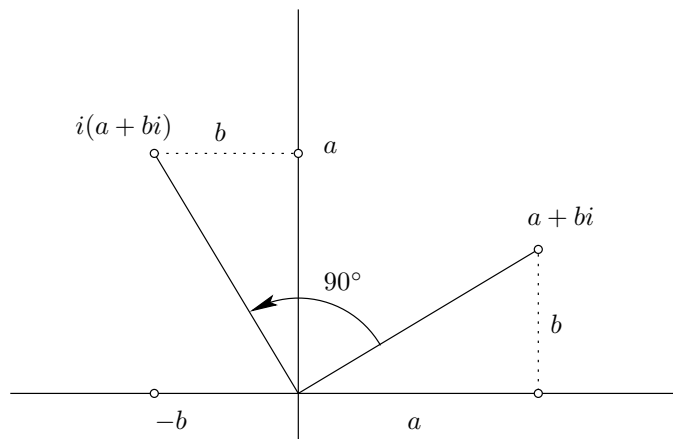
Figure 3. Multiplication of a + bi by i .
