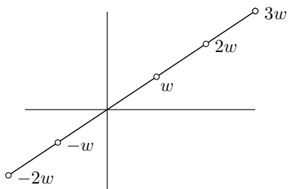
Figure 4. Multiplication of a real and a complex number
