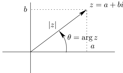
Figure 1. A complex number.
