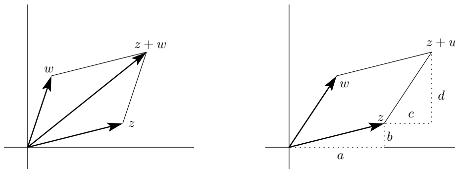
Figure 2. Addition of z = a + bi and w = c + di
