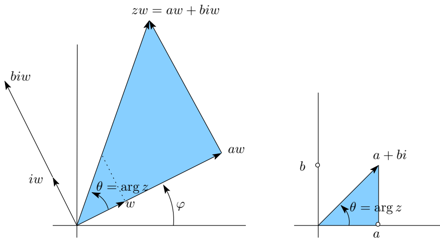
Figure 5. Multiplication of two complex numbers
